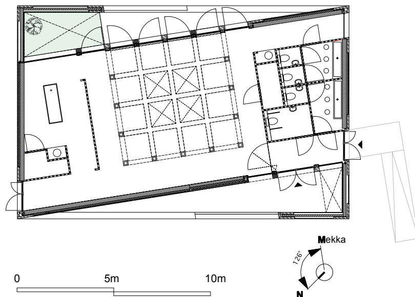
beganegron 1:200
