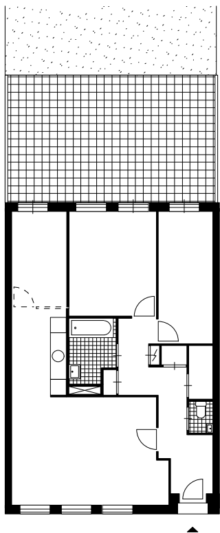
Woningtype B (bg) - GBO: 81,6m 2
