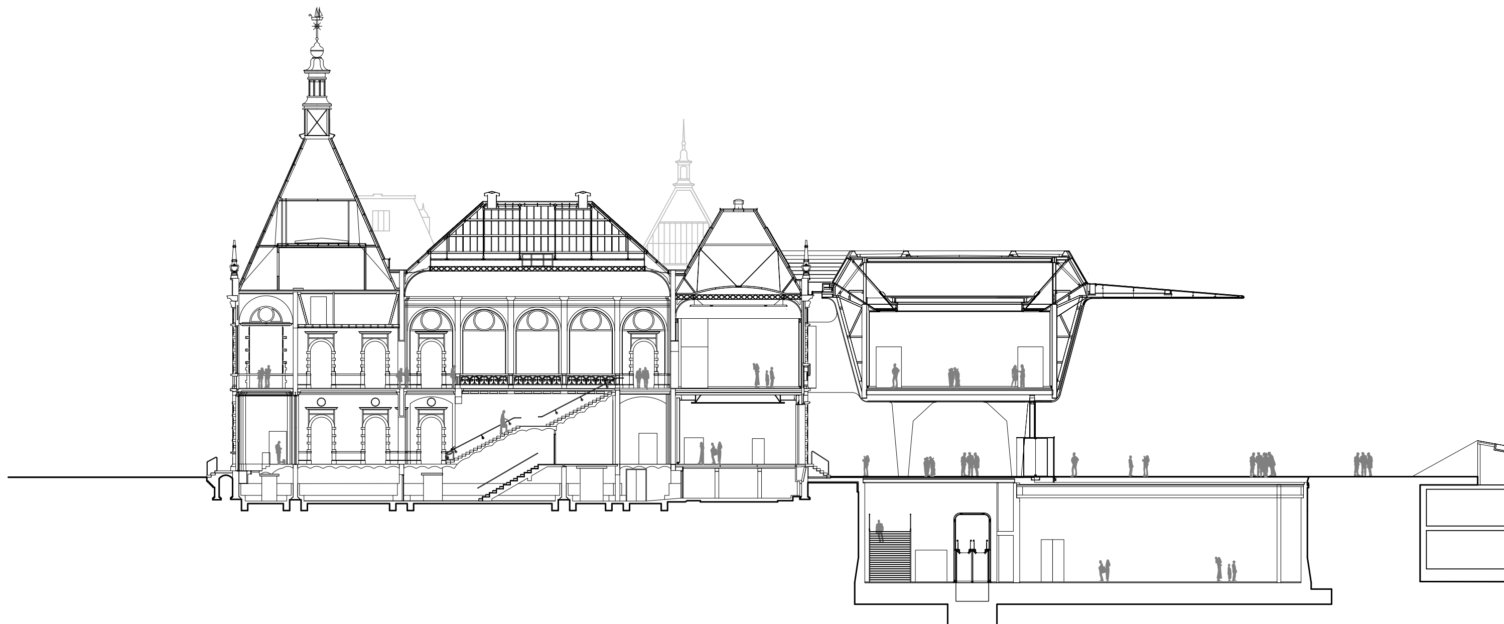
Cross section
