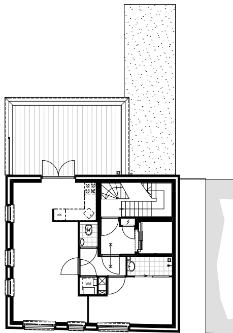
bel-etage
