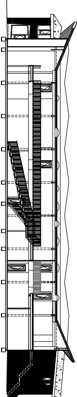
LANGSDOORSNED E
