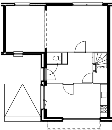
540/345-3-vs begane grond
