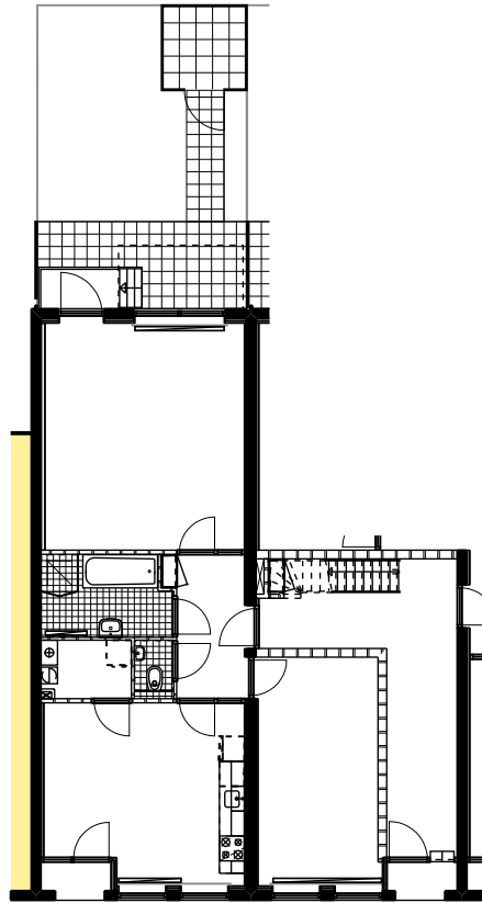
BEGANE GROND WONINGTYPE A1
