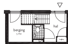
begane grond type A1 gbo: 114.0 m²
