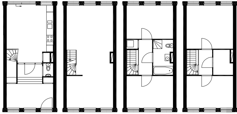
begane grond type 1
