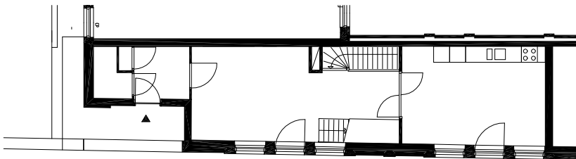
begane grond type 3
