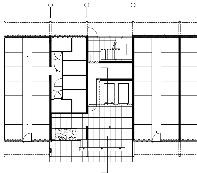
BEGANE-GROND
