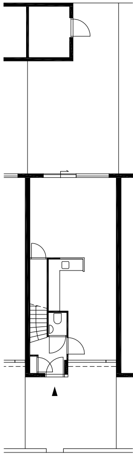
begane grond type A1
