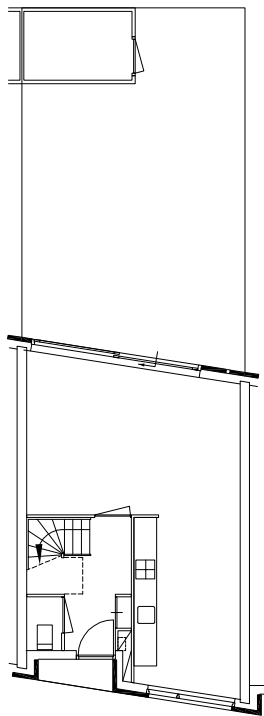
type C, begane grond
