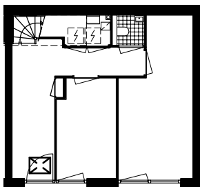
Type A, begane grond
