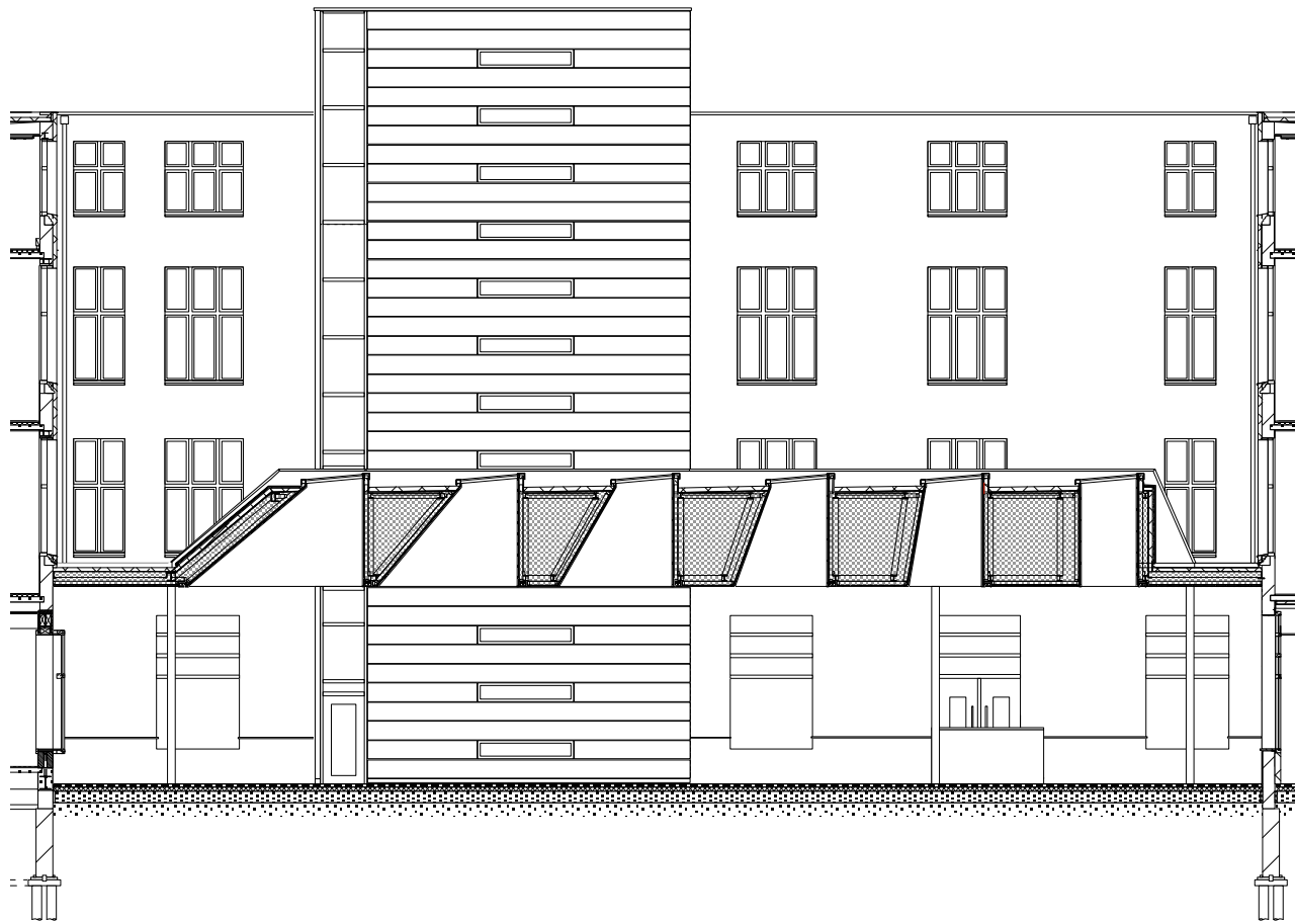
DOORSNEDE RESTAURANT 1:200
