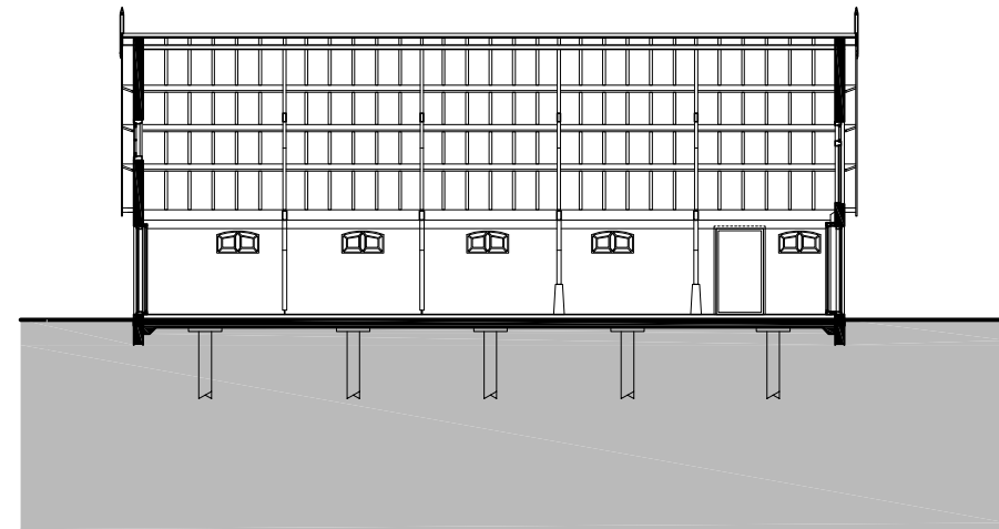
doorsnede restaurant
