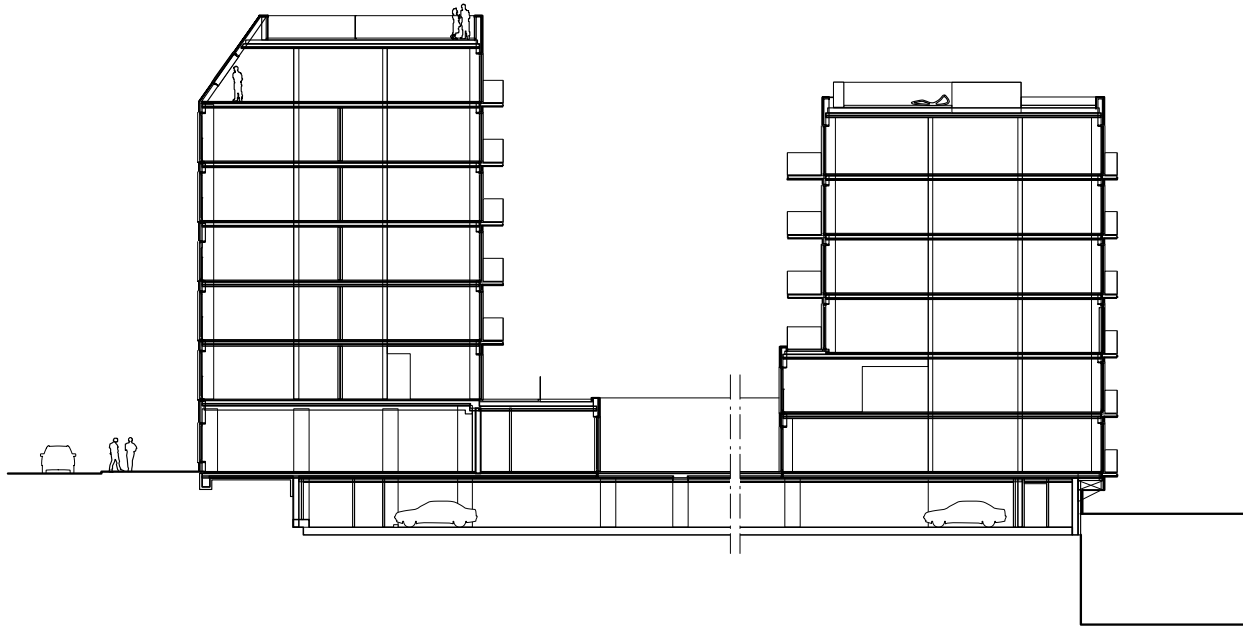
SECTION 1:400
