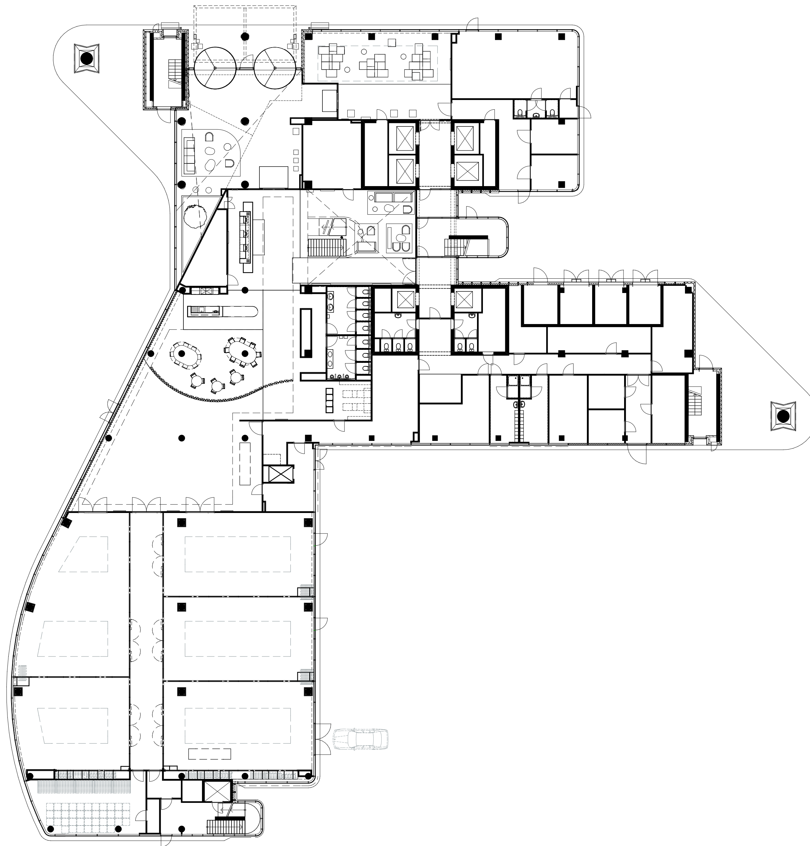
Begane grond 1:200
