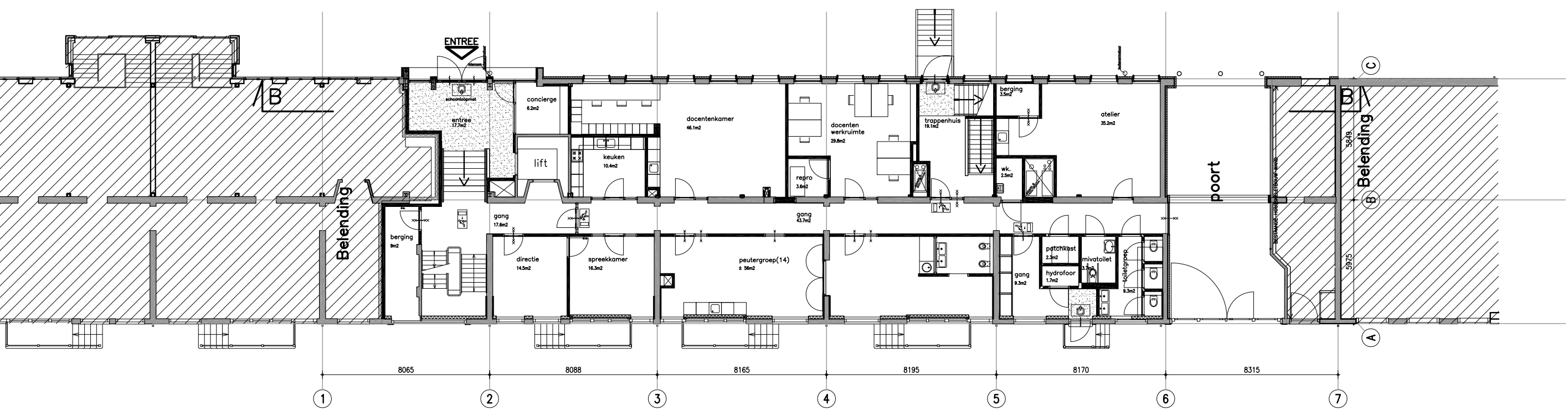
BEL-ETAGE 438.9 m2 BVO incl. poort 63 m2 BVO POORT
